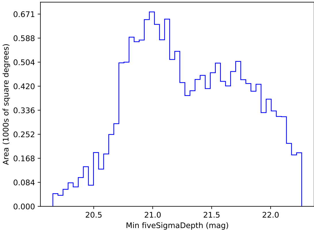
too_elab_r256_d2_griz_v3.4_10yrs WFD z band: Min fiveSigmaDepth
