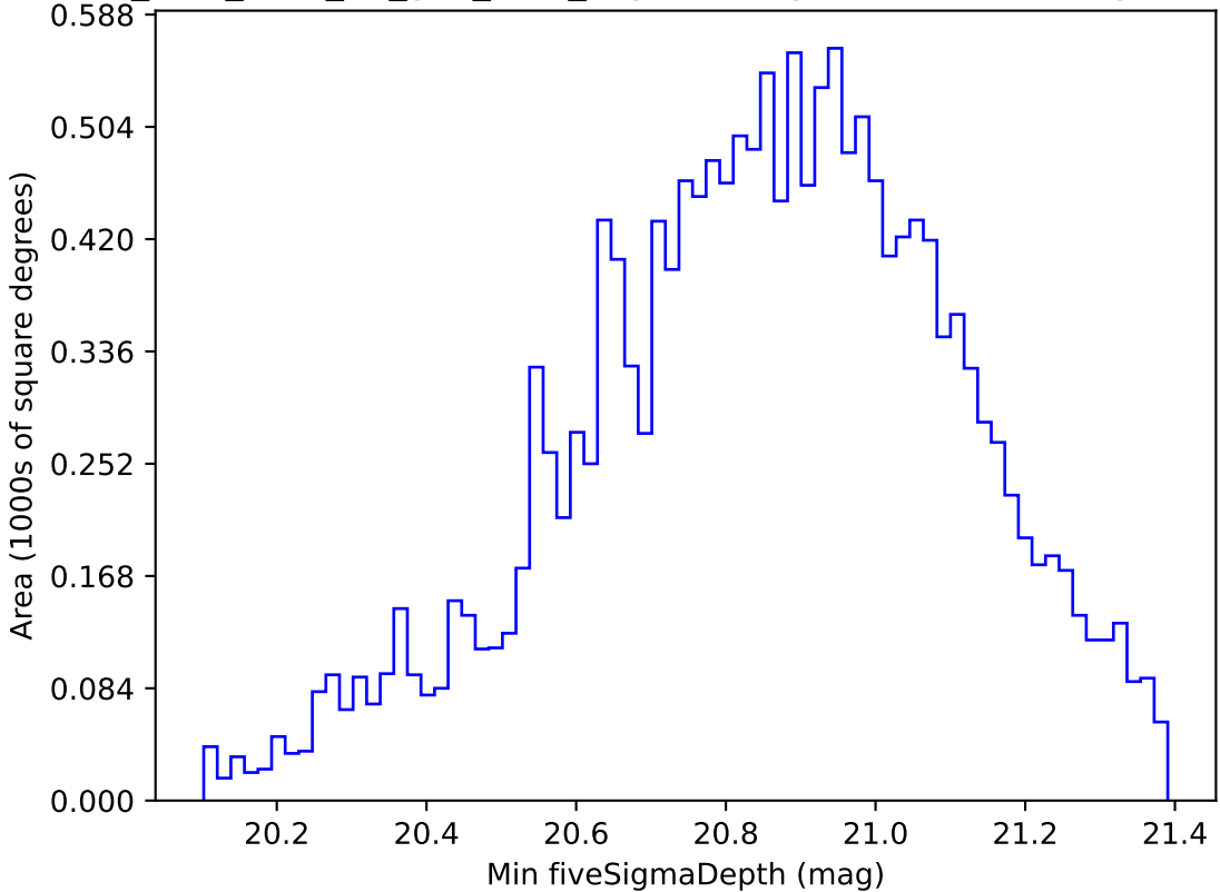
too_elab_r256_d2_griz_v3.4_10yrs WFD y band: Min fiveSigmaDepth
