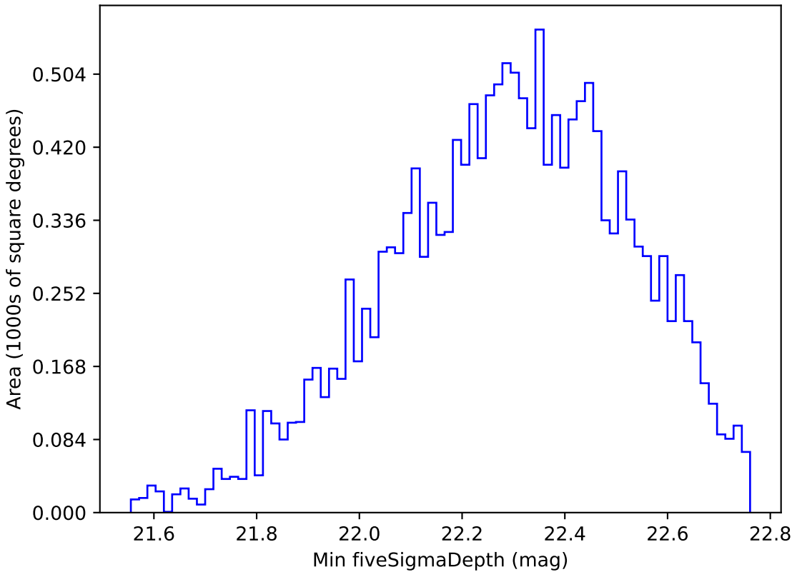
too_elab_r256_d2_griz_v3.4_10yrs WFD u band: Min fiveSigmaDepth
