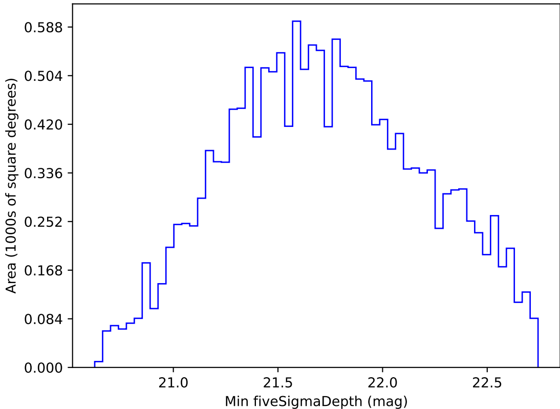
too_elab_r256_d2_griz_v3.4_10yrs WFD i band: Min fiveSigmaDepth
