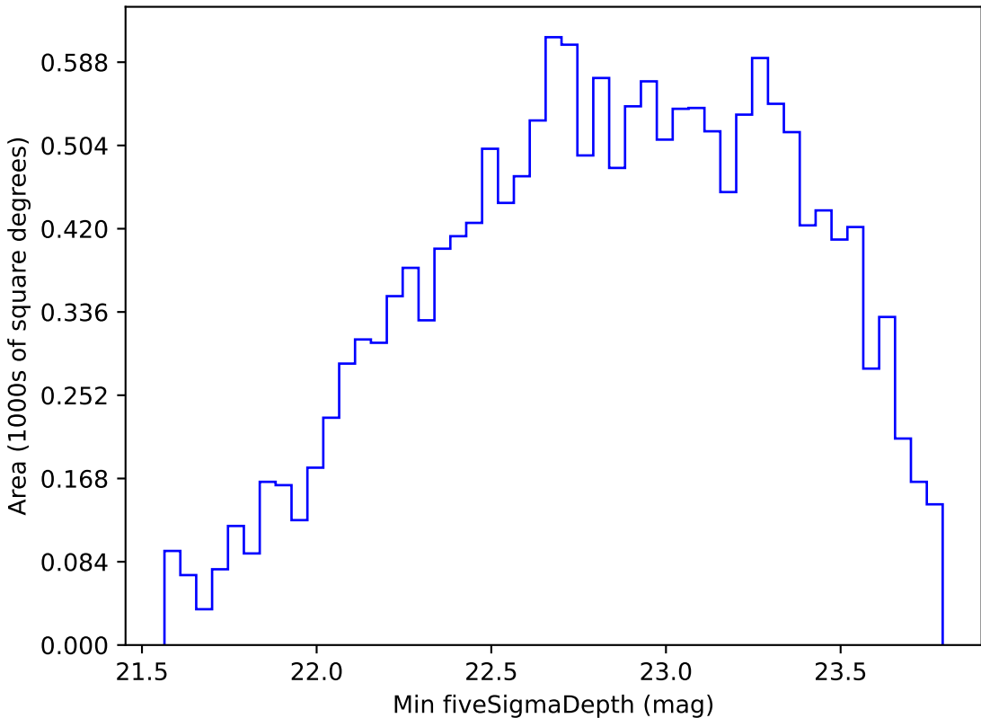
too_elab_r256_d2_griz_v3.4_10yrs WFD g band: Min fiveSigmaDepth
