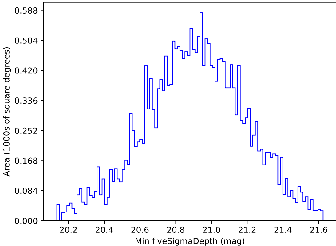
too_elab_r256_d2_griz_v3.4_10yrs All sky y band: Min fiveSigmaDepth
