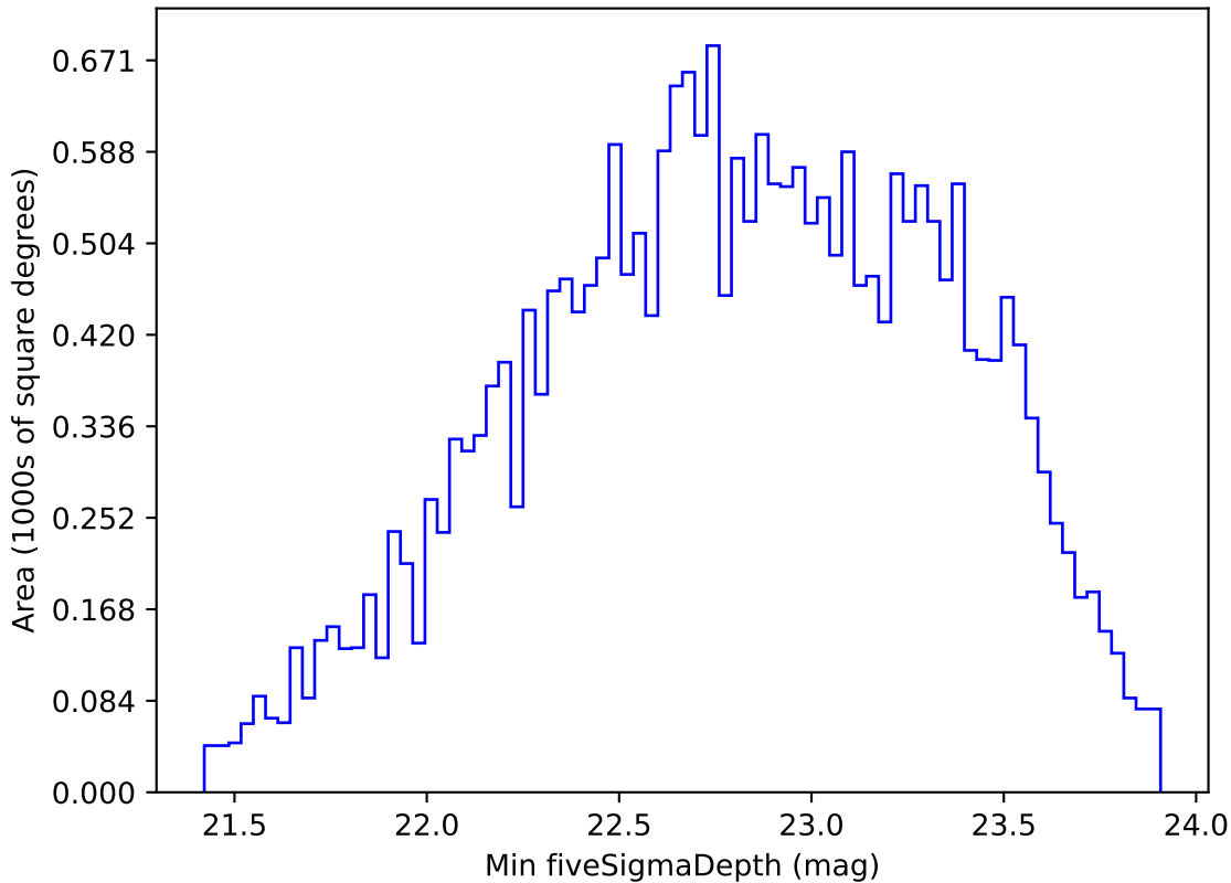
too_elab_r256_d2_griz_v3.4_10yrs All sky g band: Min fiveSigmaDepth
