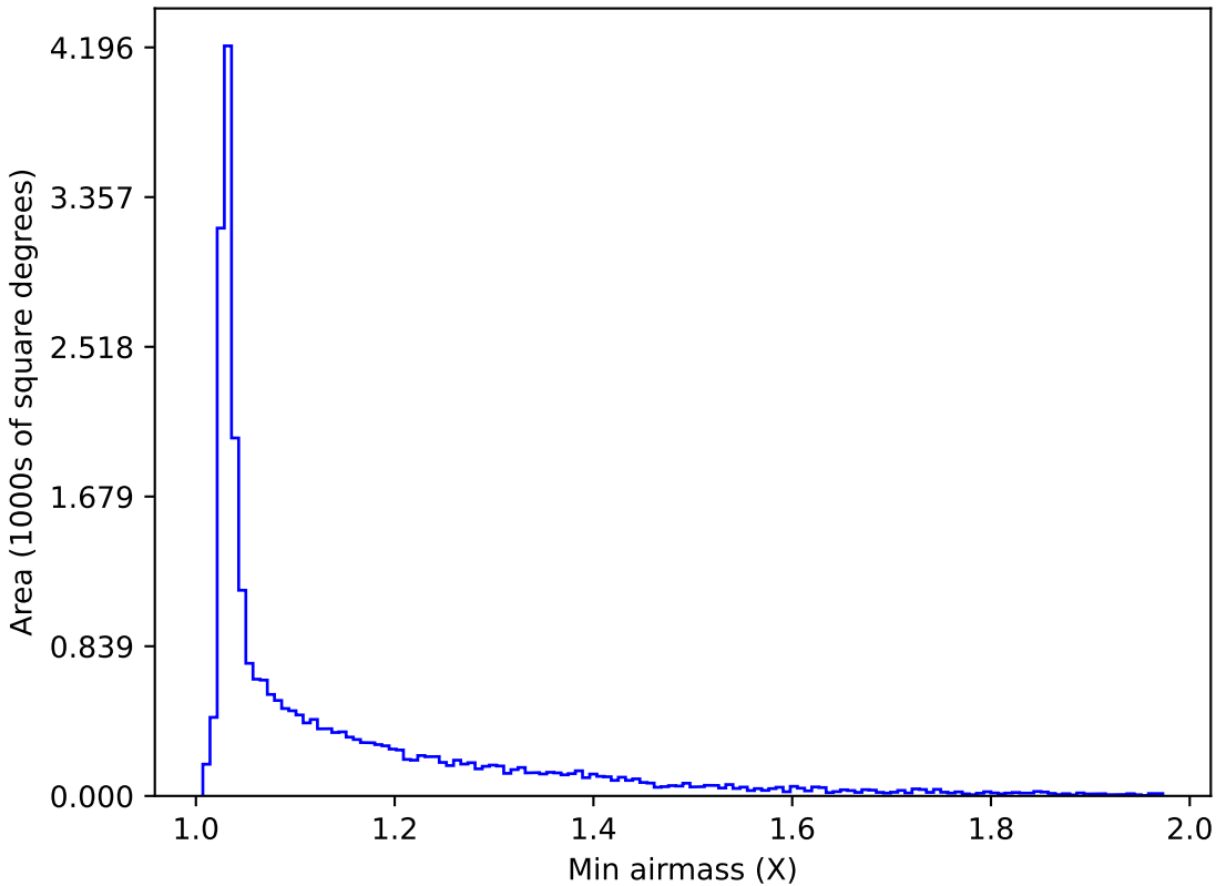
too_elab_r256_d2_griz_v3.4_10yrs Yr 1 all bands: Min airmass
