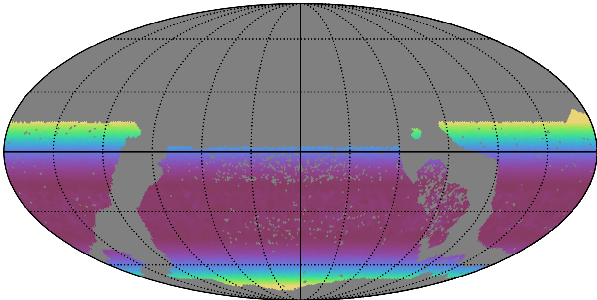
too_elab_r256_d2_griz_v3.4_10yrs WFD y band: Min airmass
