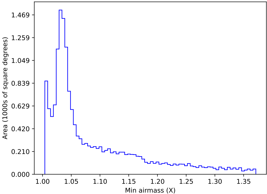
too_elab_r256_d2_griz_v3.4_10yrs WFD g band: Min airmass
