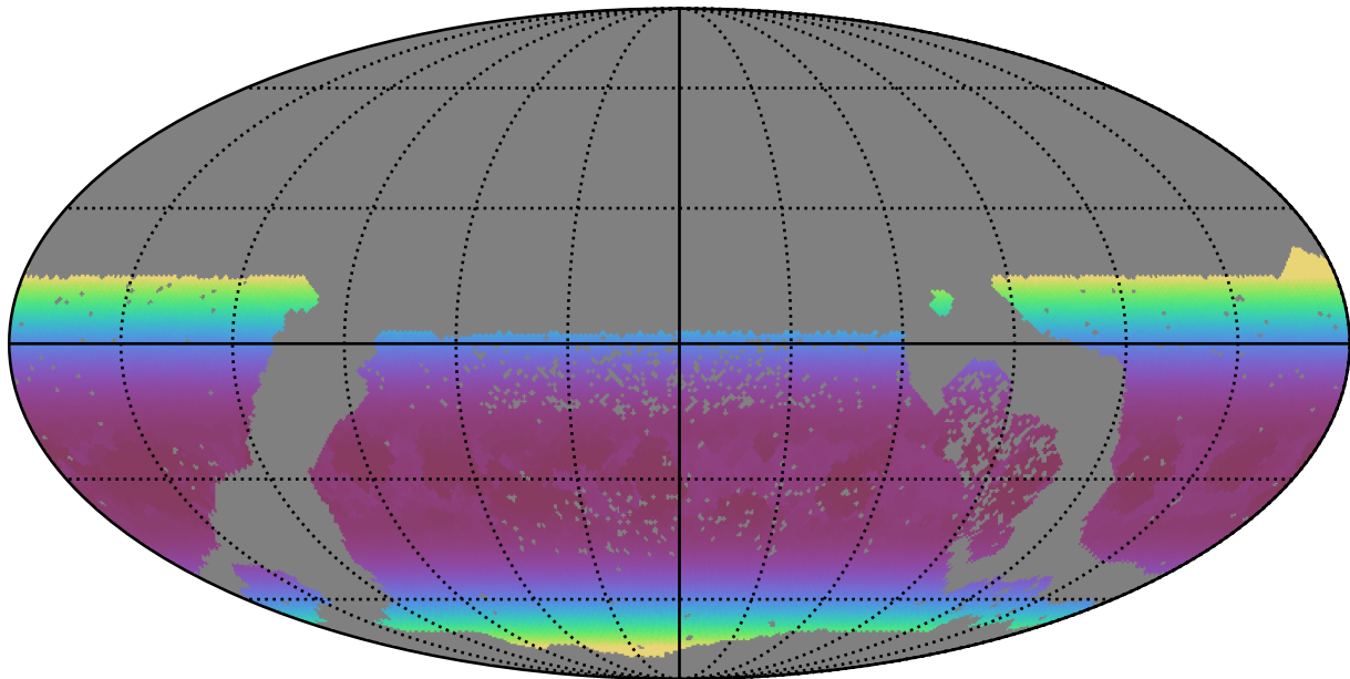
too_elab_r256_d2_griz_v3.4_10yrs WFD all bands: Min airmass
