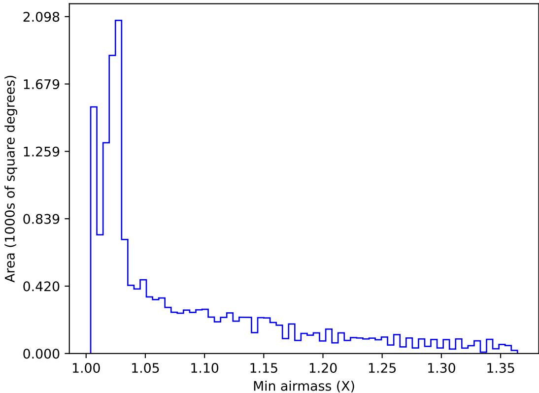
too_elab_r256_d2_griz_v3.4_10yrs WFD all bands: Min airmass
