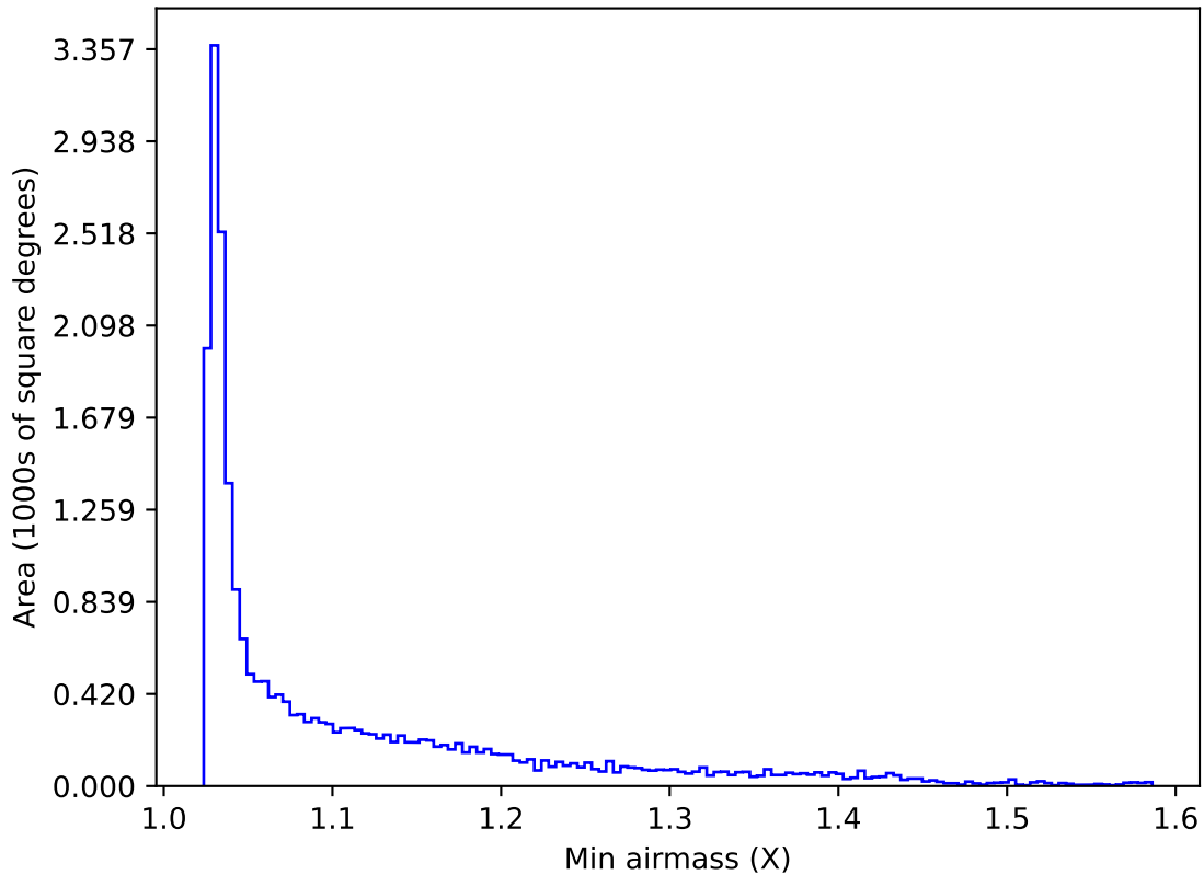
too_elab_r256_d2_griz_v3.4_10yrs All sky y band: Min airmass
