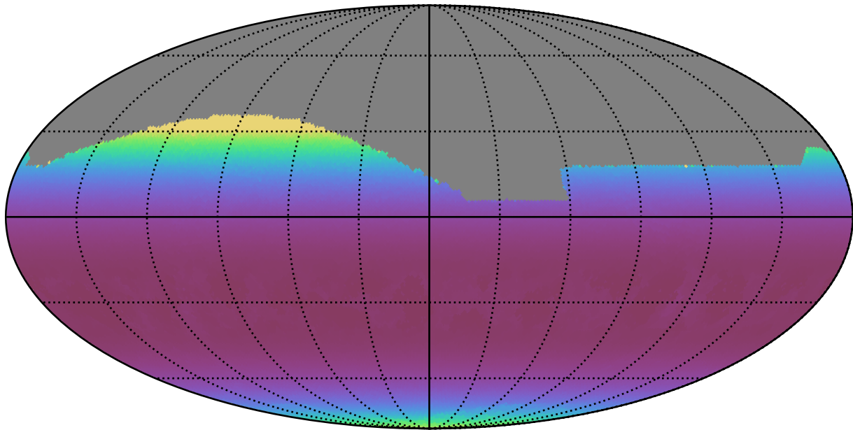
too_elab_r256_d2_griz_v3.4_10yrs All sky r band: Min airmass
