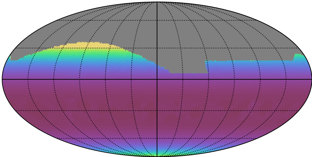
too_elab_r256_d2_griz_v3.4_10yrs All sky i band: Min airmass
