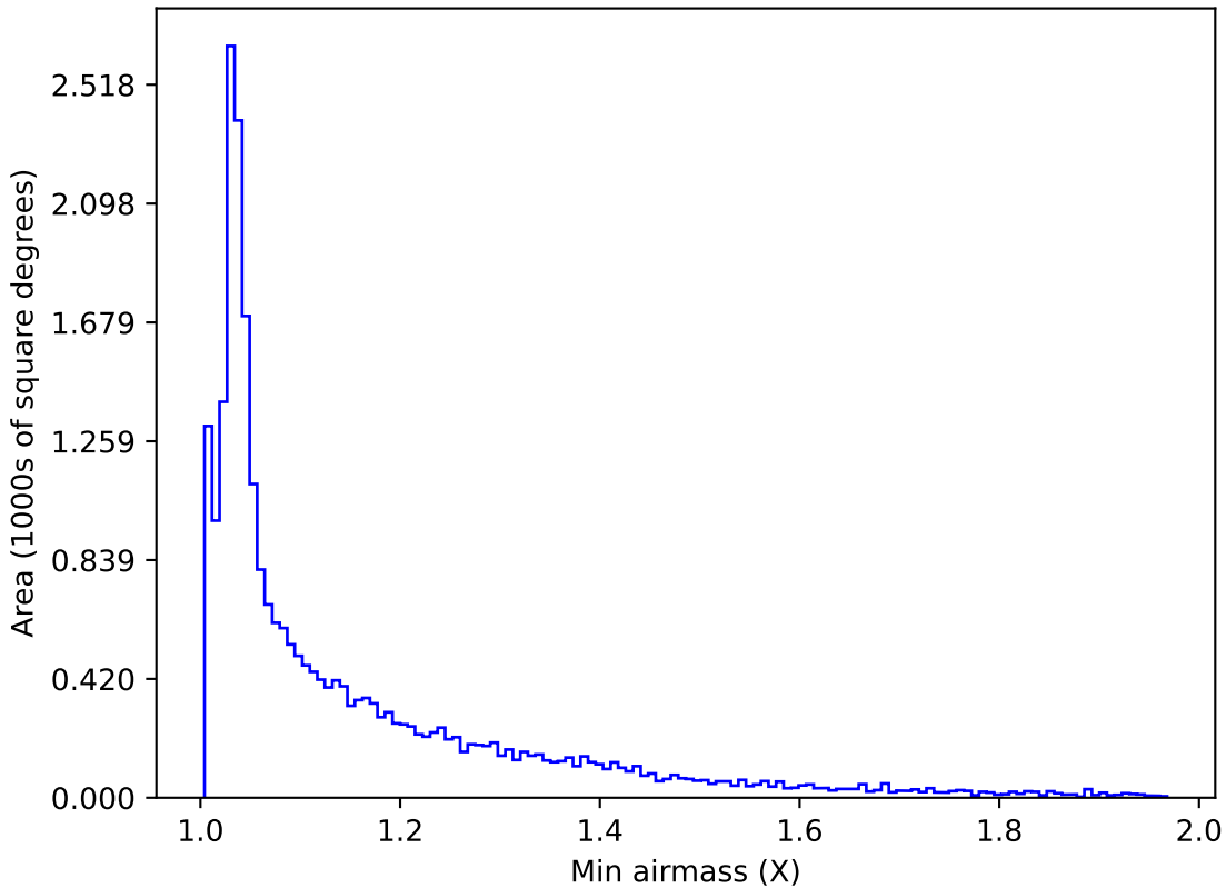
too_elab_r256_d2_griz_v3.4_10yrs All sky g band: Min airmass
