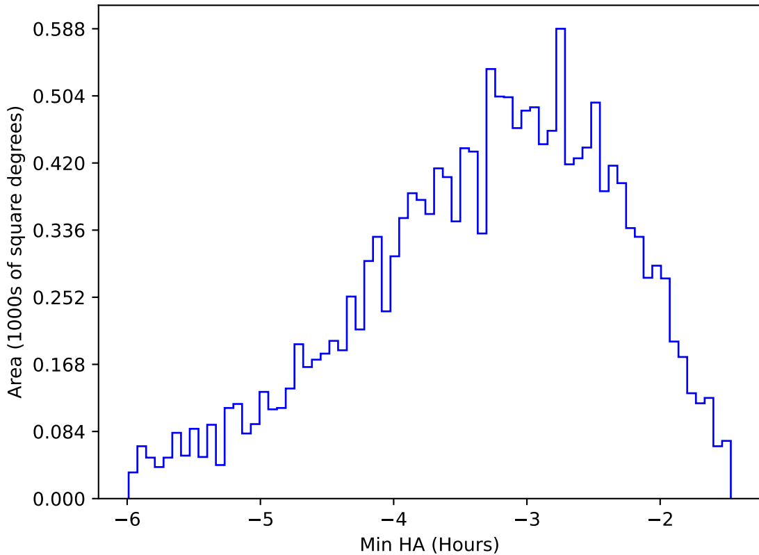
too_elab_r256_d2_griz_v3.4_10yrs WFD u band: Min HA
