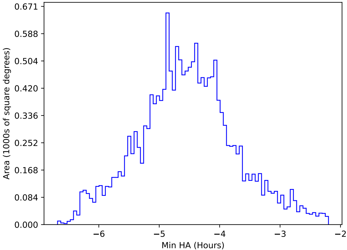
too_elab_r256_d2_griz_v3.4_10yrs WFD i band: Min HA
