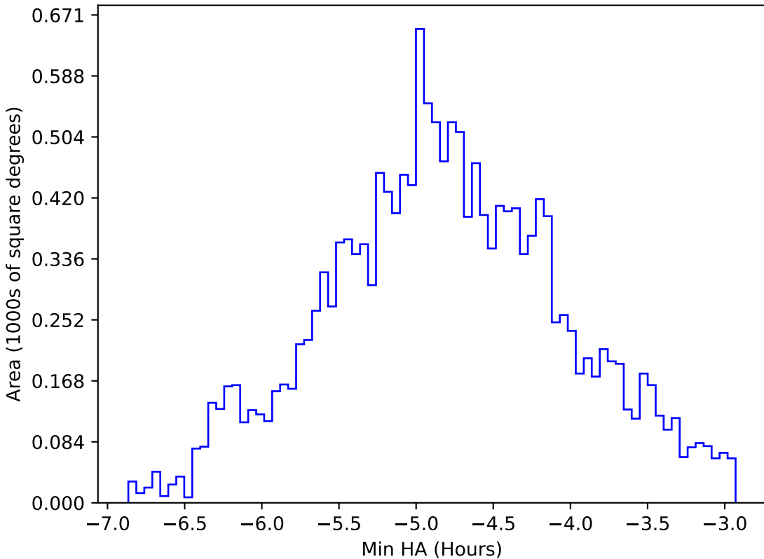
too_elab_r256_d2_griz_v3.4_10yrs WFD all bands: Min HA
