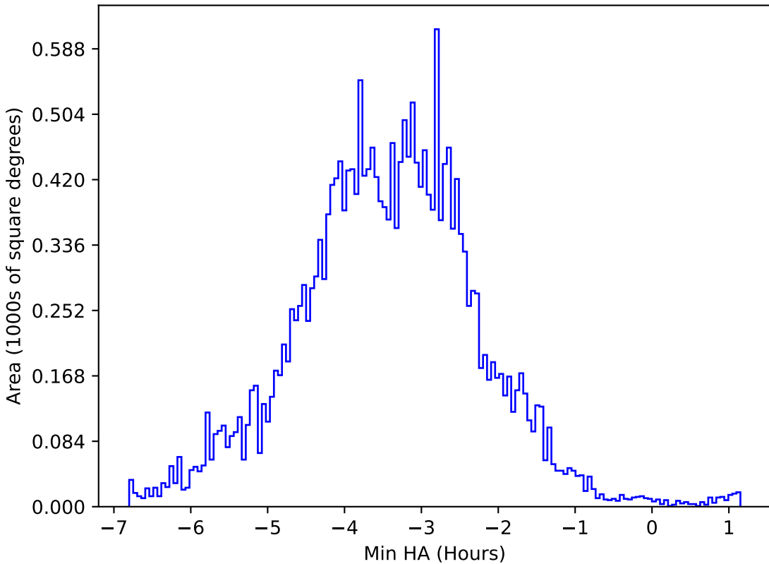
too_elab_r256_d2_griz_v3.4_10yrs All sky y band: Min HA
