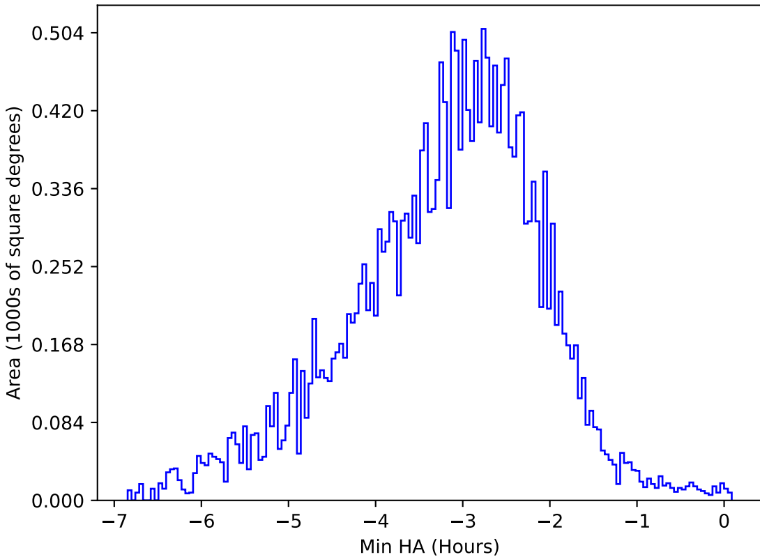
too_elab_r256_d2_griz_v3.4_10yrs All sky u band: Min HA
