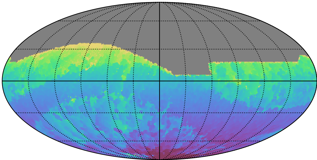
too_elab_r256_d2_griz_v3.4_10yrs All sky r band: Min HA
