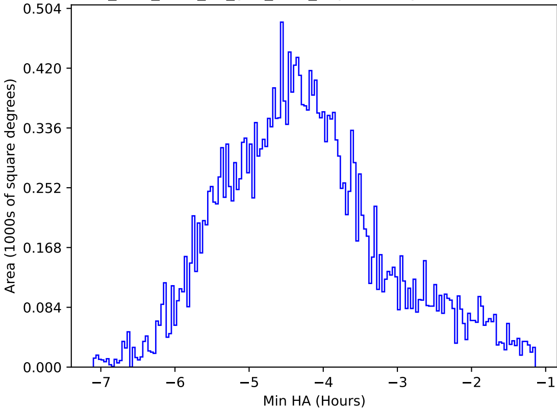
too_elab_r256_d2_griz_v3.4_10yrs All sky r band: Min HA
