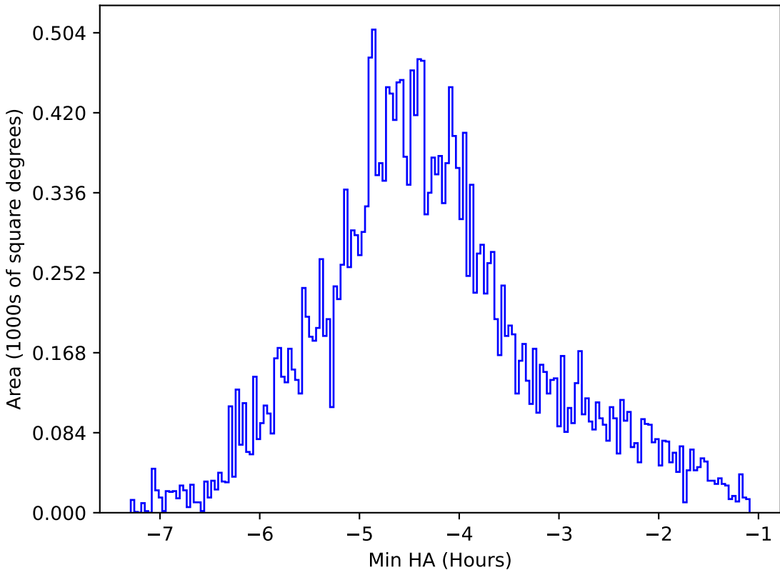
too_elab_r256_d2_griz_v3.4_10yrs All sky i band: Min HA
