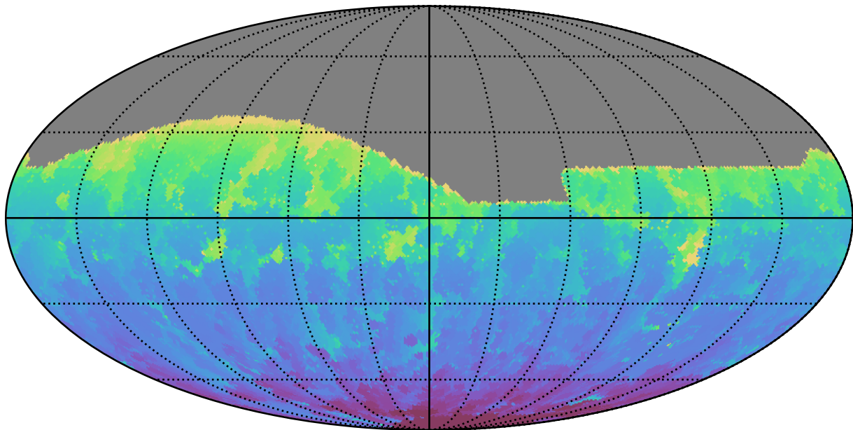
too_elab_r256_d2_griz_v3.4_10yrs All sky g band: Min HA
