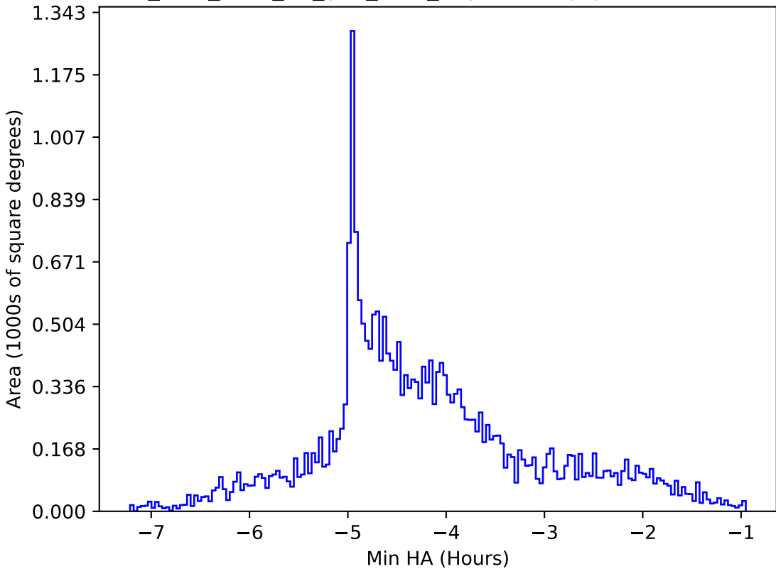
too_elab_r256_d2_griz_v3.4_10yrs All sky g band: Min HA
