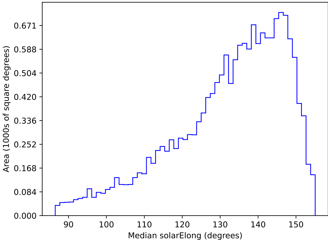
too_elab_r256_d2_griz_v3.4_10yrs WFD u band: Median solarElong
