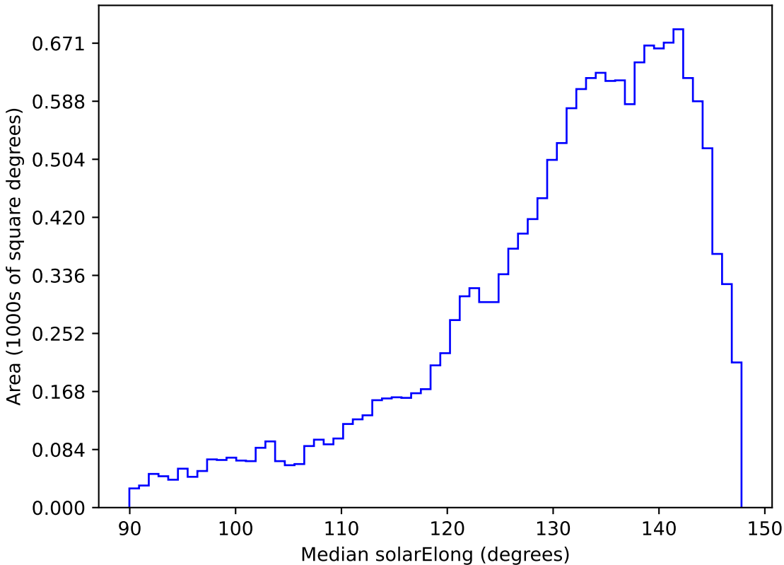
too_elab_r256_d2_griz_v3.4_10yrs WFD r band: Median solarElong
