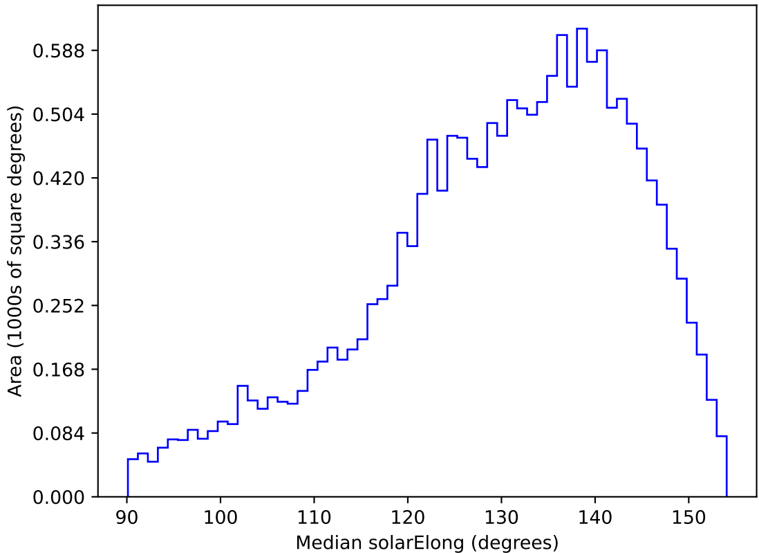
too_elab_r256_d2_griz_v3.4_10yrs WFD g band: Median solarElong
