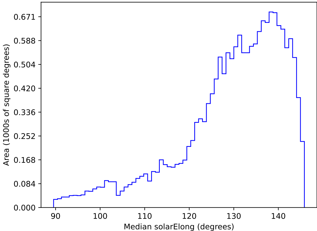
too_elab_r256_d2_griz_v3.4_10yrs WFD all bands: Median solarElong
