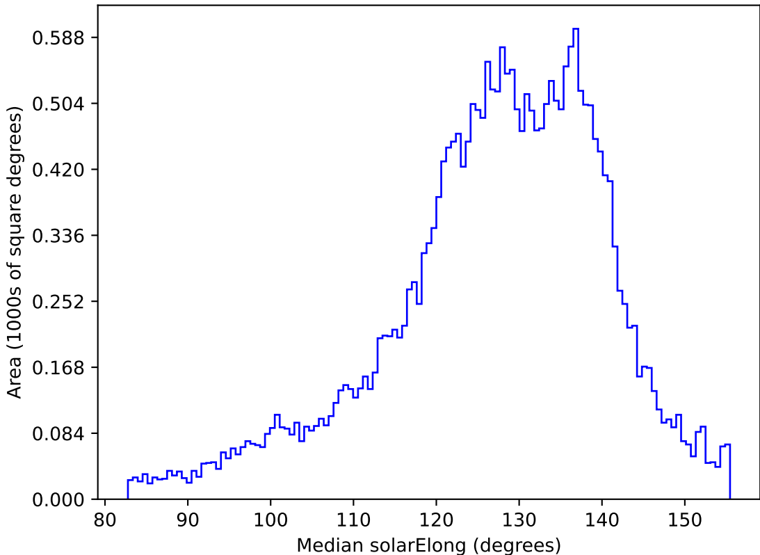
too_elab_r256_d2_griz_v3.4_10yrs All sky z band: Median solarElong
