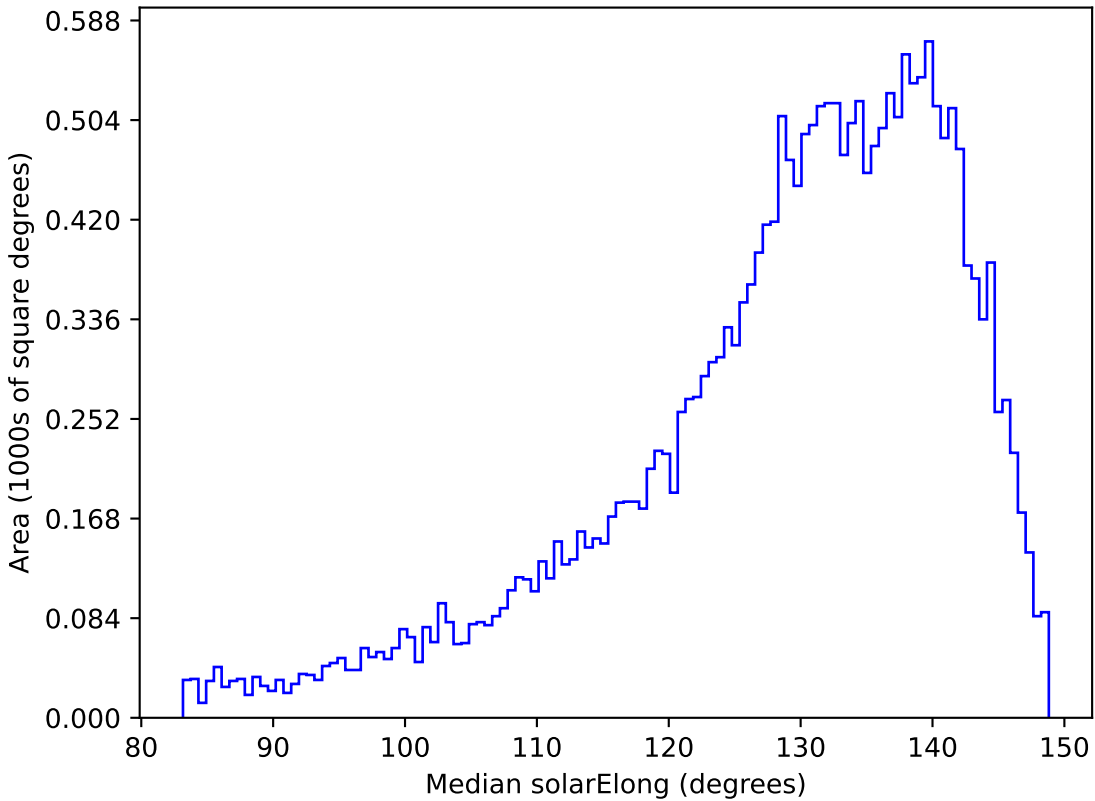
too_elab_r256_d2_griz_v3.4_10yrs All sky y band: Median solarElong
