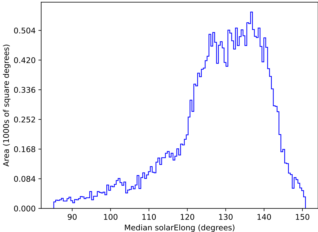
too_elab_r256_d2_griz_v3.4_10yrs All sky i band: Median solarElong
