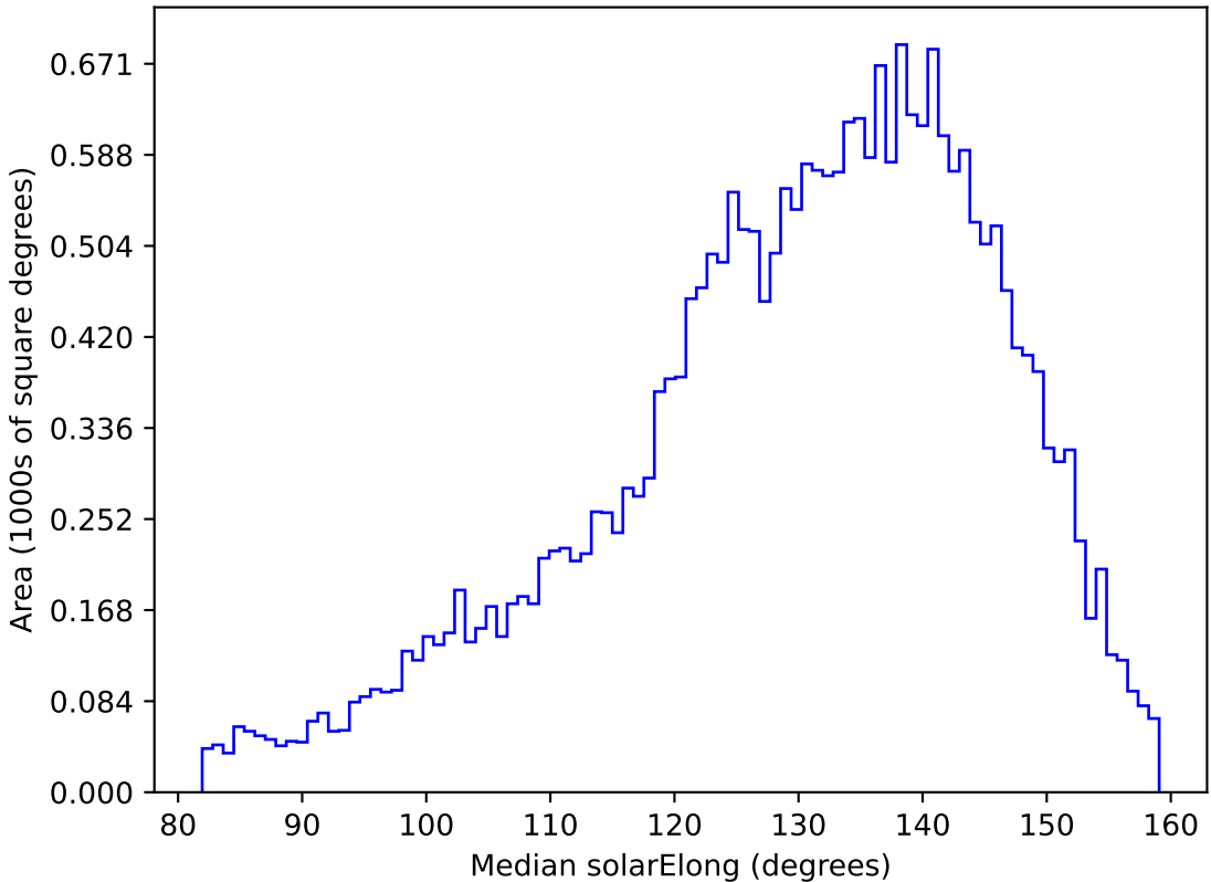
too_elab_r256_d2_griz_v3.4_10yrs All sky g band: Median solarElong
