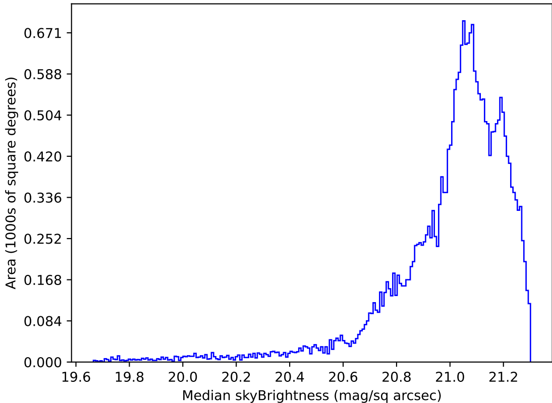
too_elab_r256_d2_griz_v3.4_10yrs Yr 1 r band: Median skyBrightness
