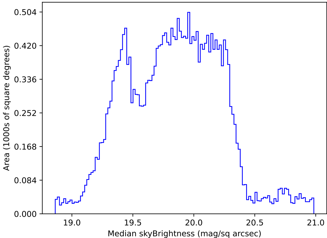
too_elab_r256_d2_griz_v3.4_10yrs Yr 1 all bands: Median skyBrightness
