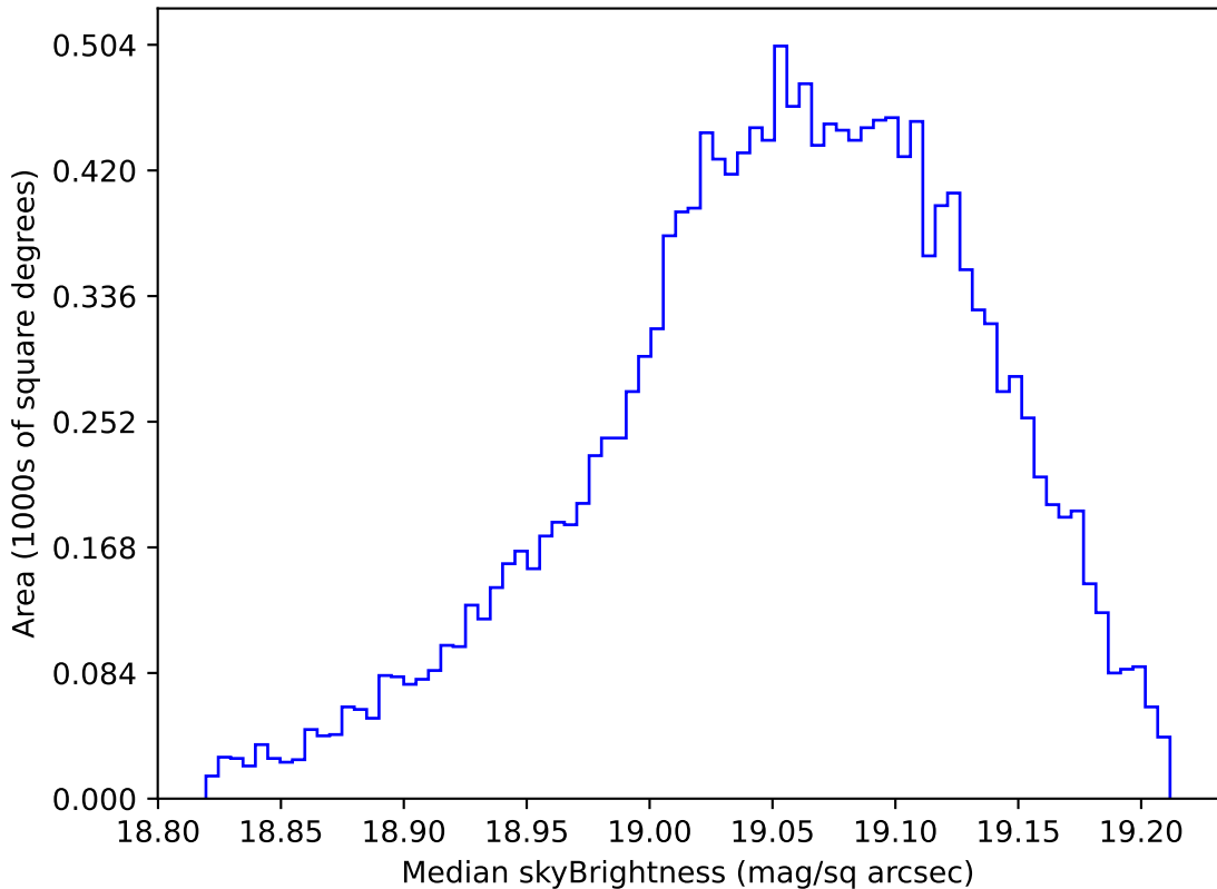
too_elab_r256_d2_griz_v3.4_10yrs WFD z band: Median skyBrightness
