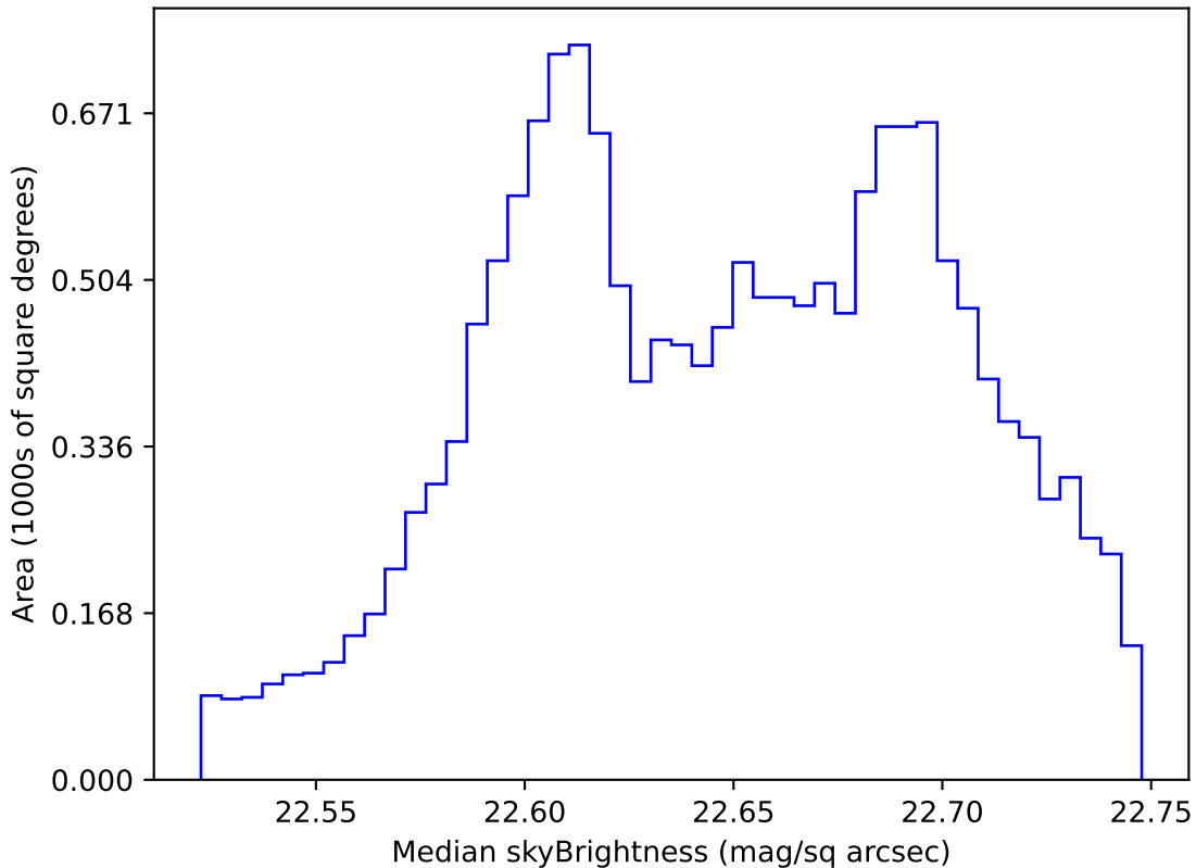
too_elab_r256_d2_griz_v3.4_10yrs WFD u band: Median skyBrightness
