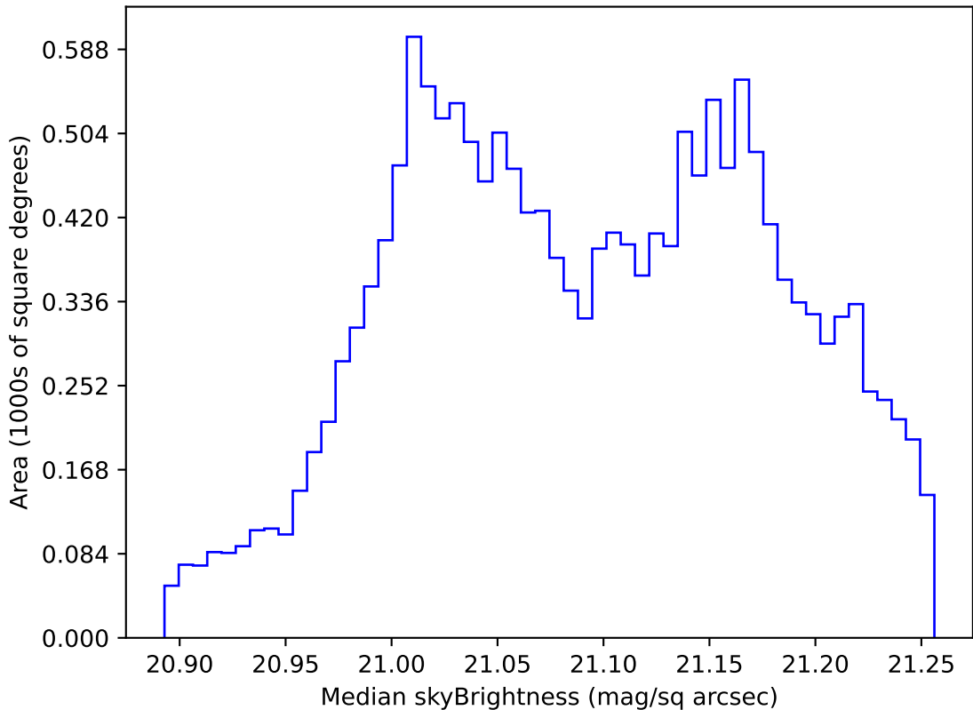
too_elab_r256_d2_griz_v3.4_10yrs WFD r band: Median skyBrightness
