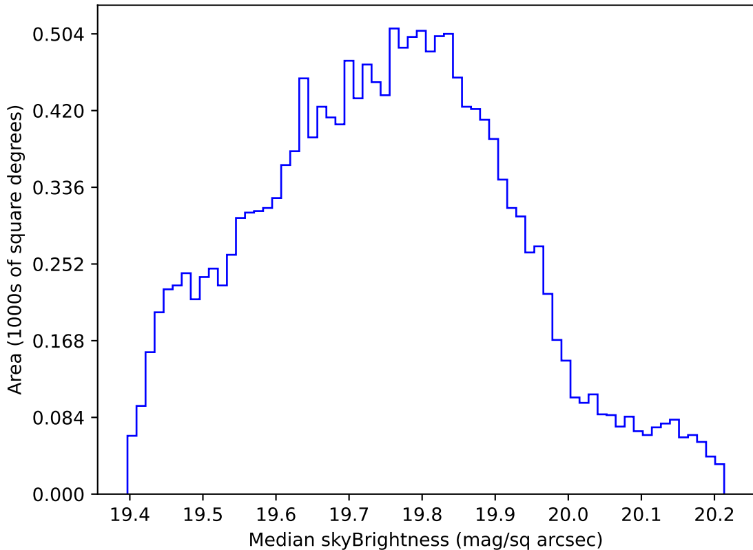
too_elab_r256_d2_griz_v3.4_10yrs WFD all bands: Median skyBrightness
