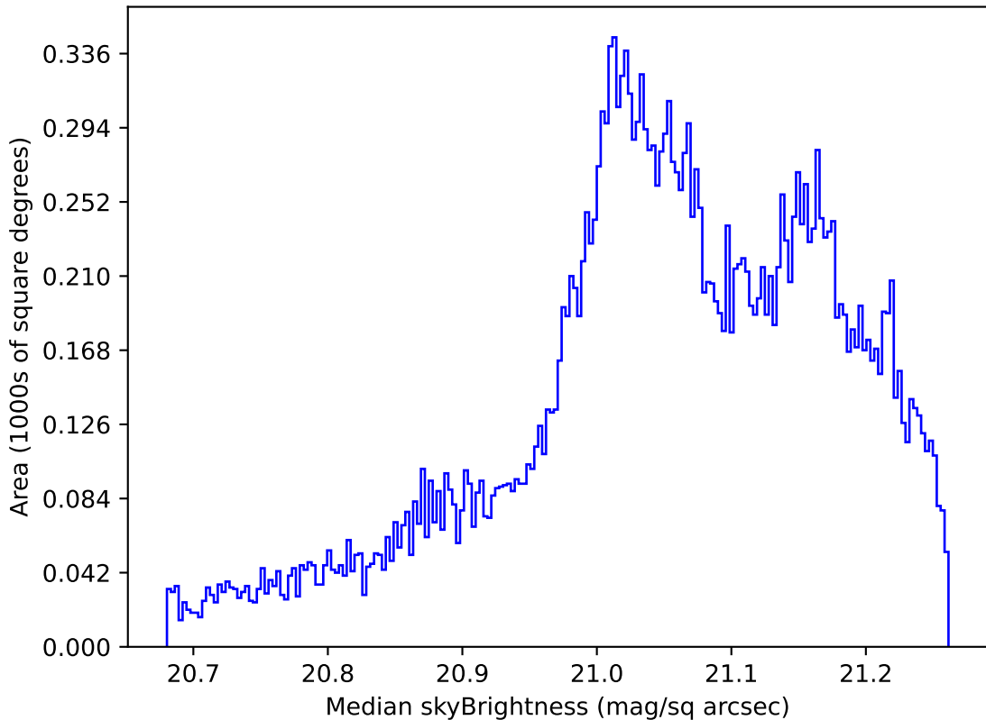
too_elab_r256_d2_griz_v3.4_10yrs All sky r band: Median skyBrightness
