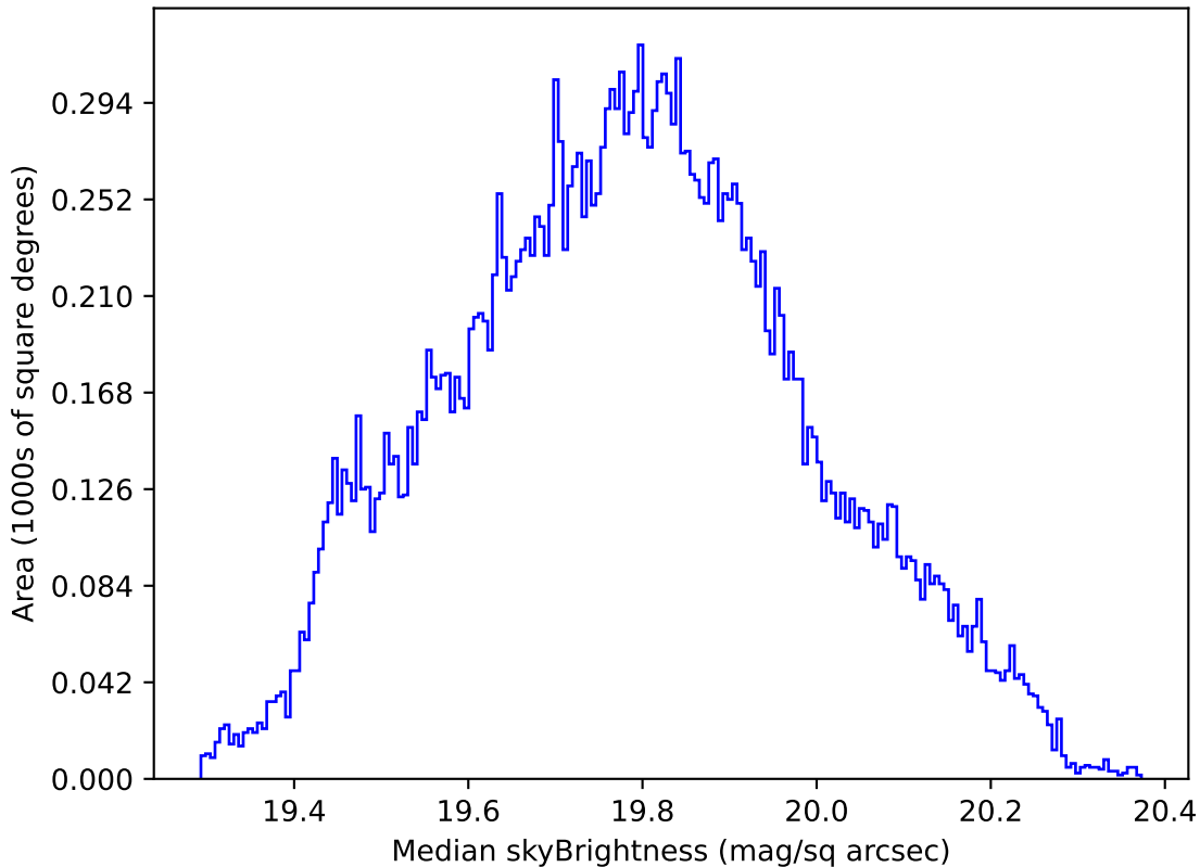
too_elab_r256_d2_griz_v3.4_10yrs All sky all bands: Median skyBrightness
