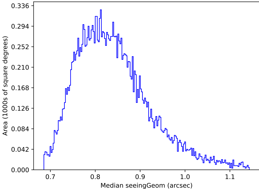
too_elab_r256_d2_griz_v3.4_10yrs Yr 1 y band: Median seeingGeom
