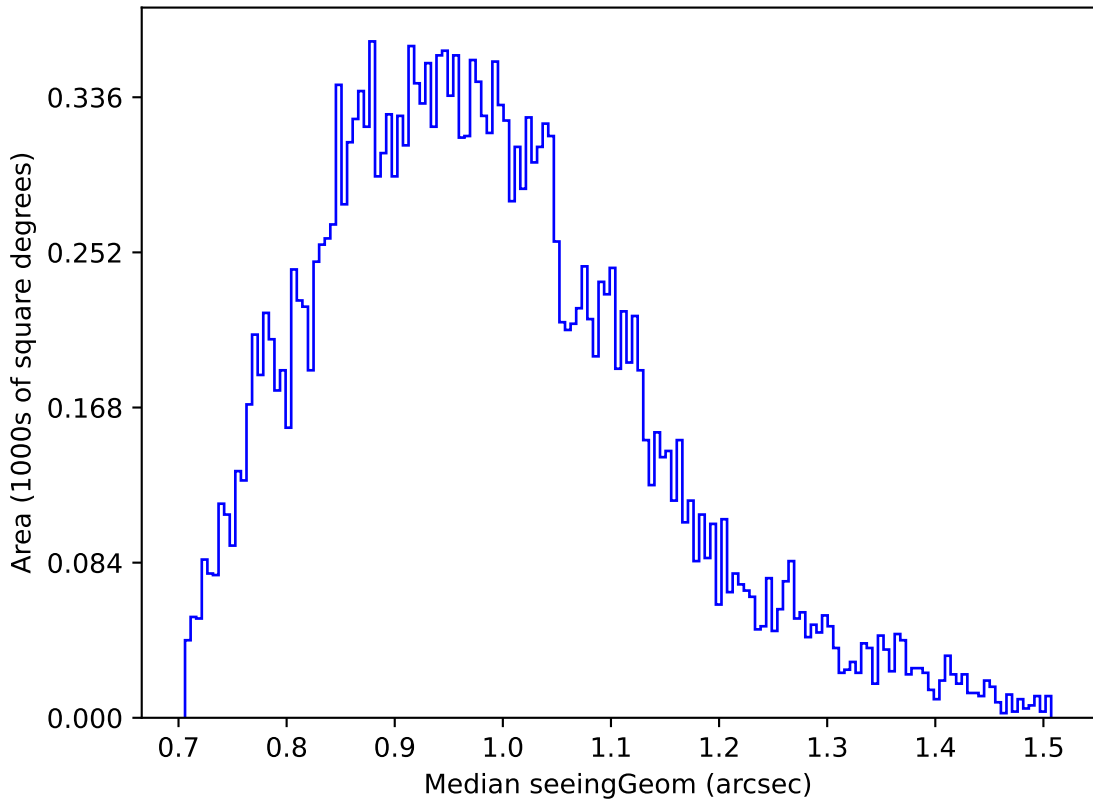
too_elab_r256_d2_griz_v3.4_10yrs Yr 1 u band: Median seeingGeom
