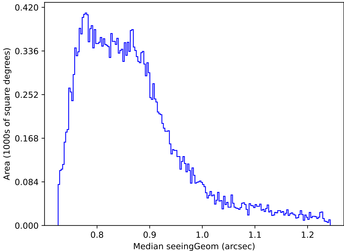
too_elab_r256_d2_griz_v3.4_10yrs Yr 1 all bands: Median seeingGeom
