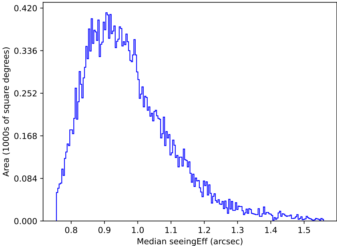
too_elab_r256_d2_griz_v3.4_10yrs Yr 1 z band: Median seeingEff
