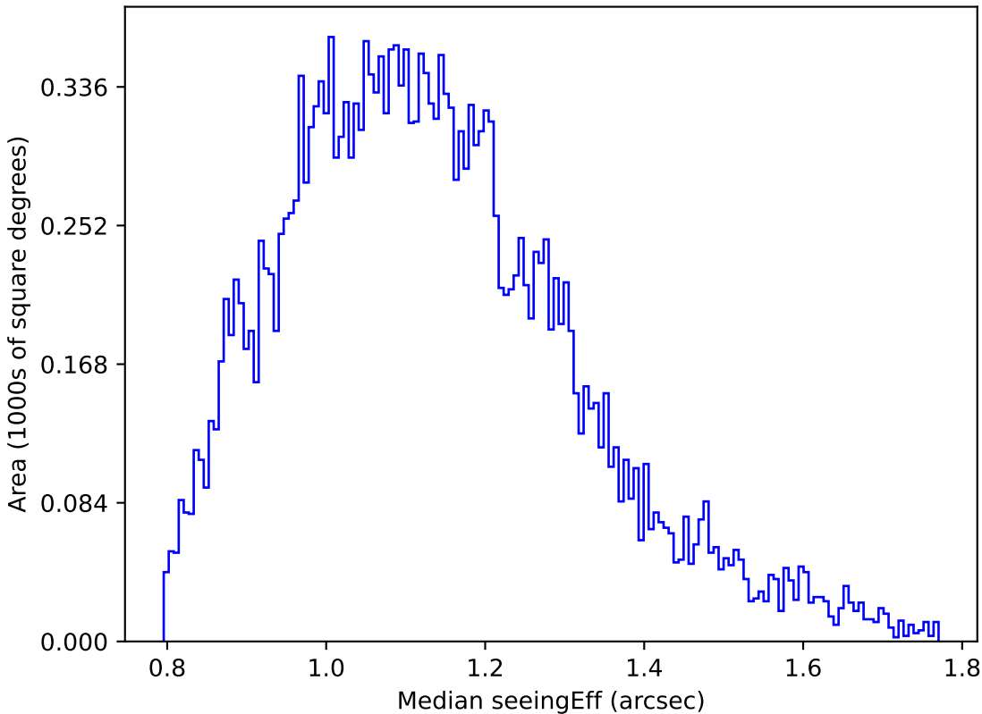
too_elab_r256_d2_griz_v3.4_10yrs Yr 1 u band: Median seeingEff
