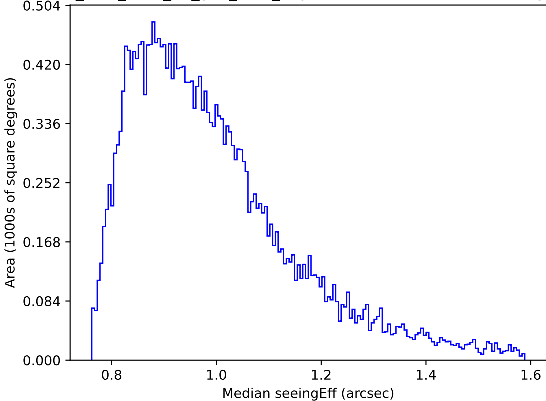
too_elab_r256_d2_griz_v3.4_10yrs Yr 1 r band: Median seeingEff
