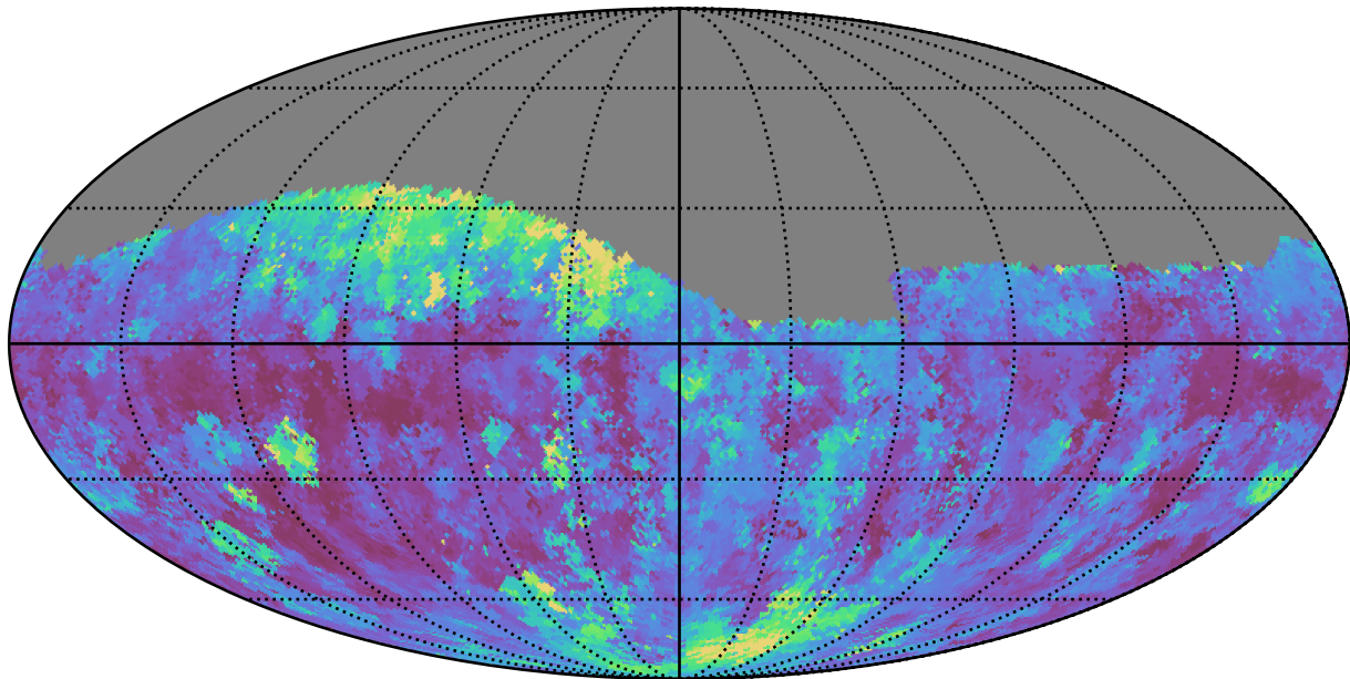
too_elab_r256_d2_griz_v3.4_10yrs Yr 1 g band: Median seeingEff
