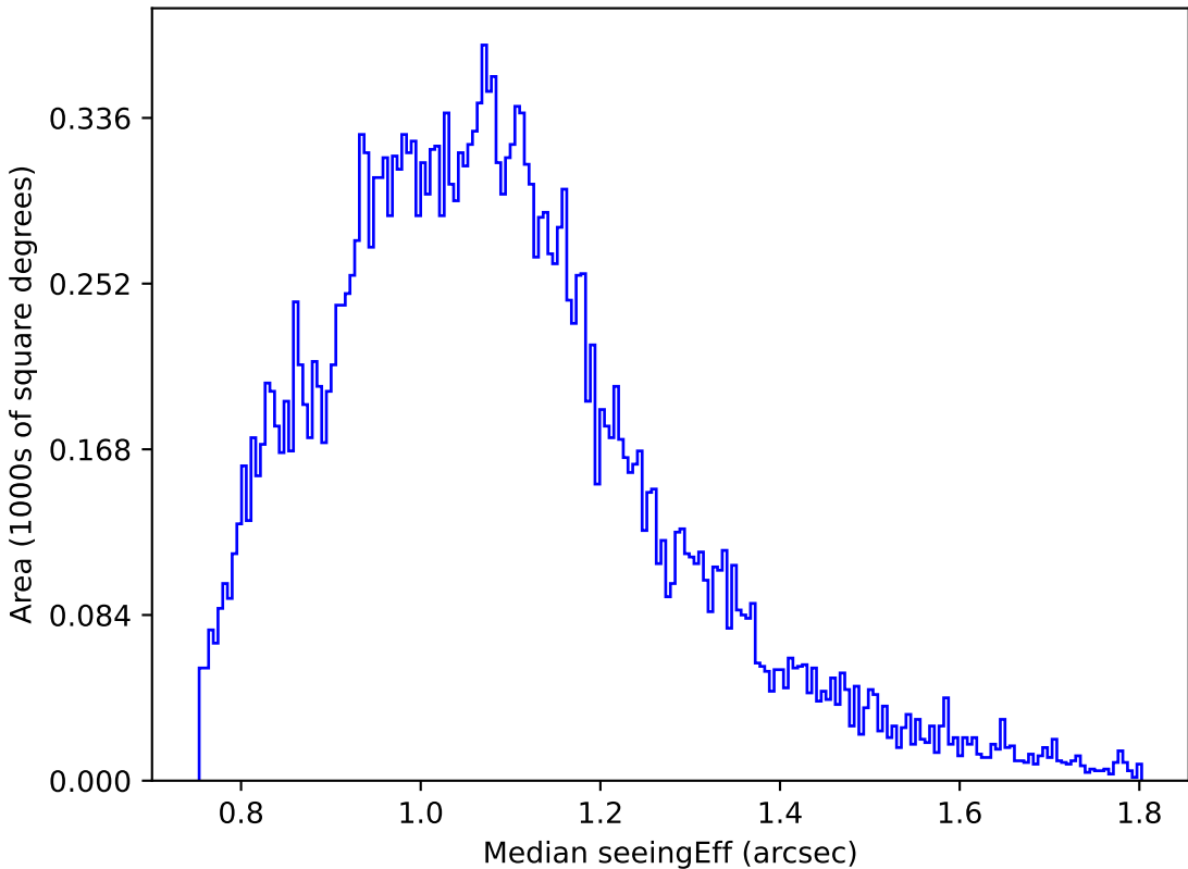
too_elab_r256_d2_griz_v3.4_10yrs Yr 1 g band: Median seeingEff
